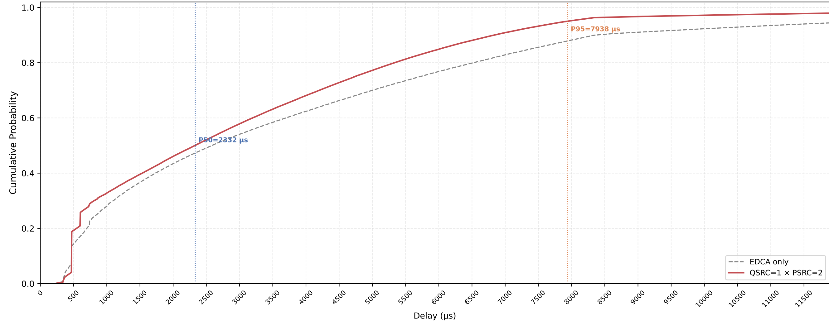
P-EDCA STA VO Delay CDF — QSRC=1 × PSRC=2 nSta=30, nPedca=30, 1Mbps, avg of 10 runs
