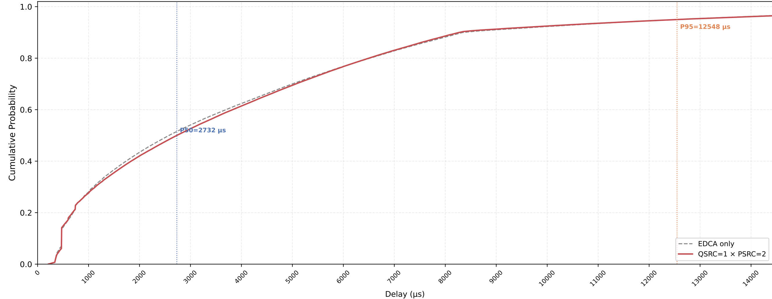
VO (all STAs) Delay CDF — QSRC=1 × PSRC=2 nSta=30, nPedca=5, 1Mbps, avg of 10 runs
