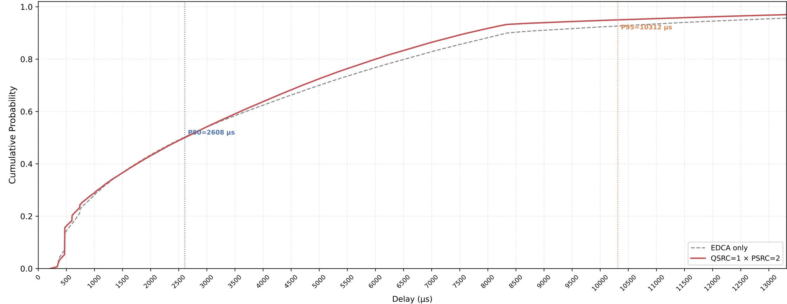
VO (all STAs) Delay CDF — QSRC=1 × PSRC=2 nSta=30, nPedca=15, 1Mbps, avg of 10 runs
