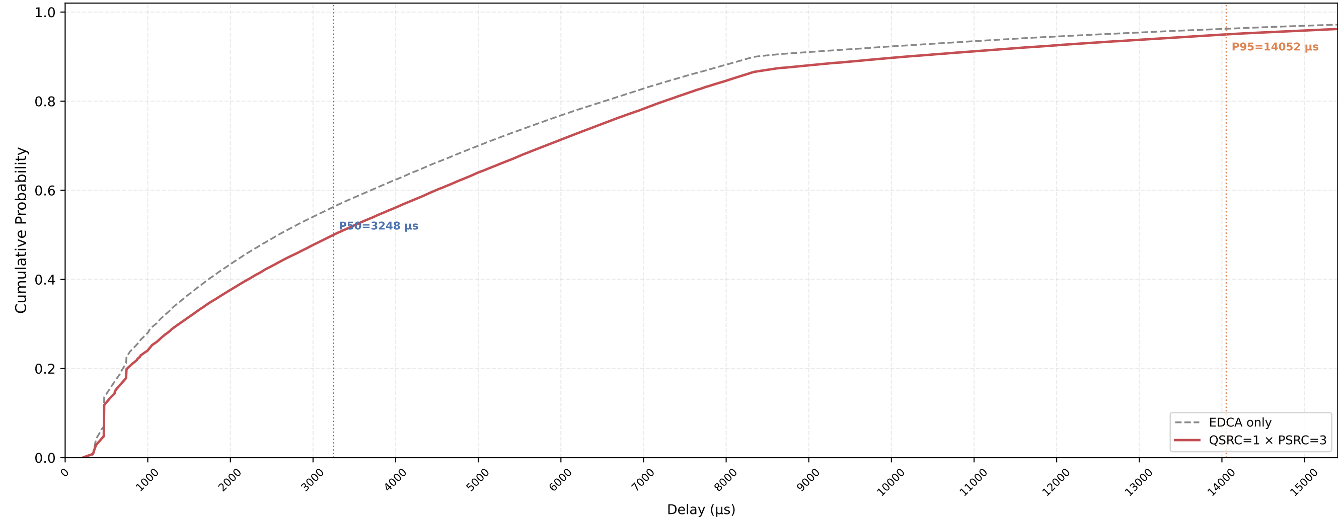
Legacy STA VO Delay CDF — QSRC=1 × PSRC=3 nSta=30, nPedca=15, 1Mbps, avg of 10 runs
