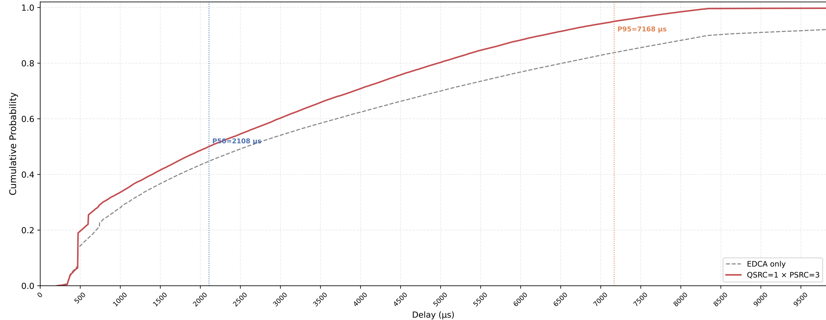
P-EDCA STA VO Delay CDF — QSRC=1 × PSRC=3 nSta=30, nPedca=5, 1Mbps, avg of 10 runs
