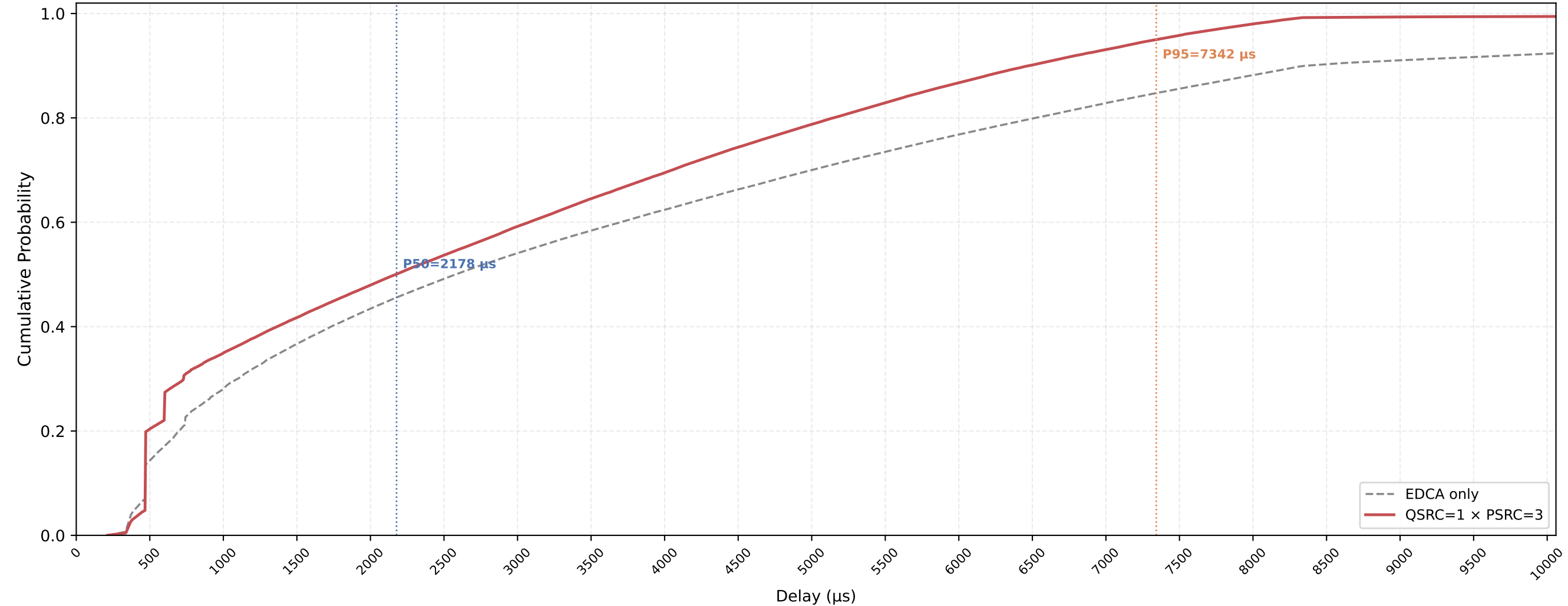
P-EDCA STA VO Delay CDF — QSRC=1 × PSRC=3 nSta=30, nPedca=15, 1Mbps, avg of 10 runs
