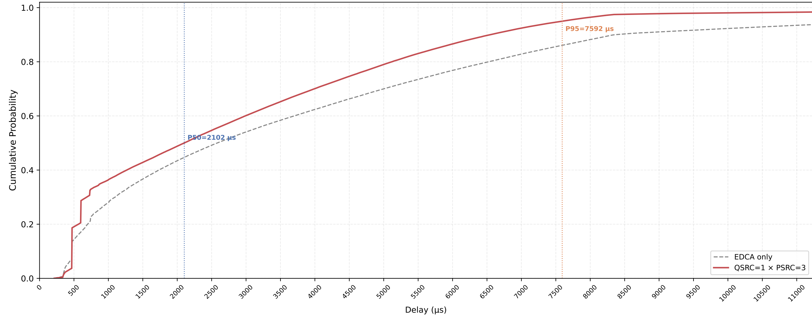
P-EDCA STA VO Delay CDF — QSRC=1 × PSRC=3 nSta=30, nPedca=30, 1Mbps, avg of 10 runs
