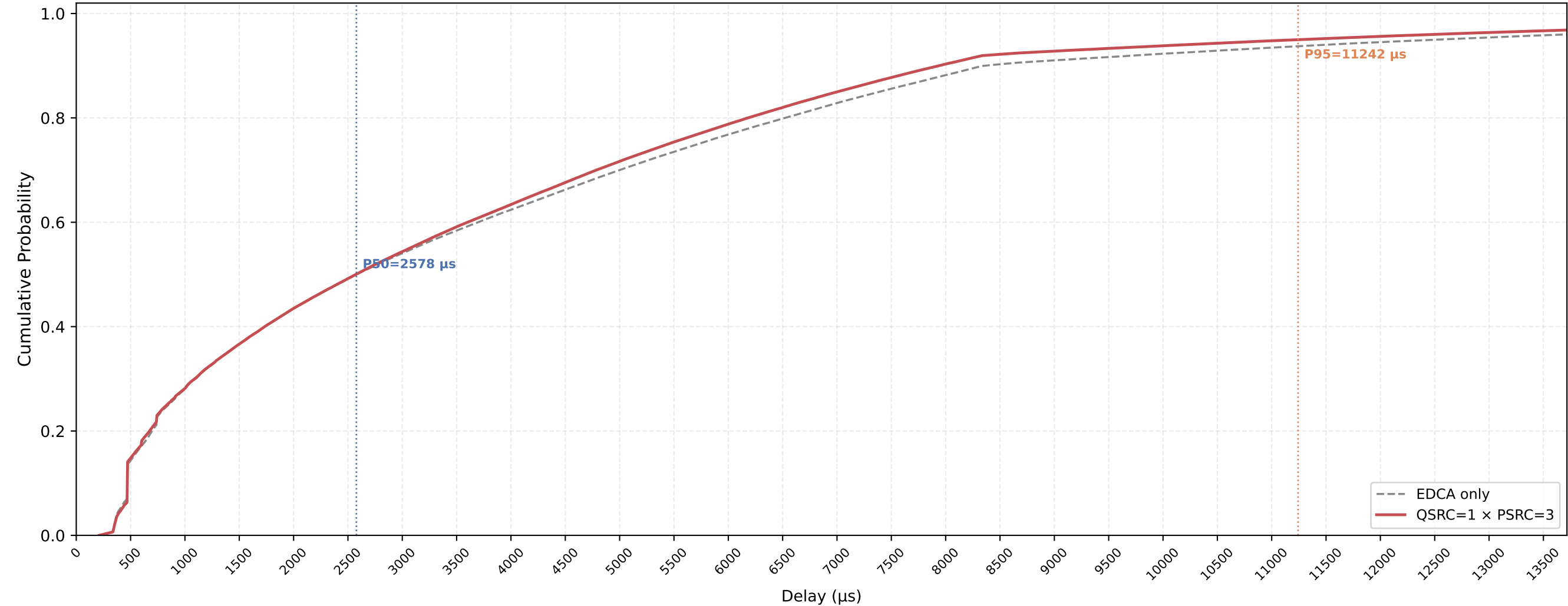
VO (all STAs) Delay CDF — QSRC=1 × PSRC=3 nSta=30, nPedca=5, 1Mbps, avg of 10 runs
