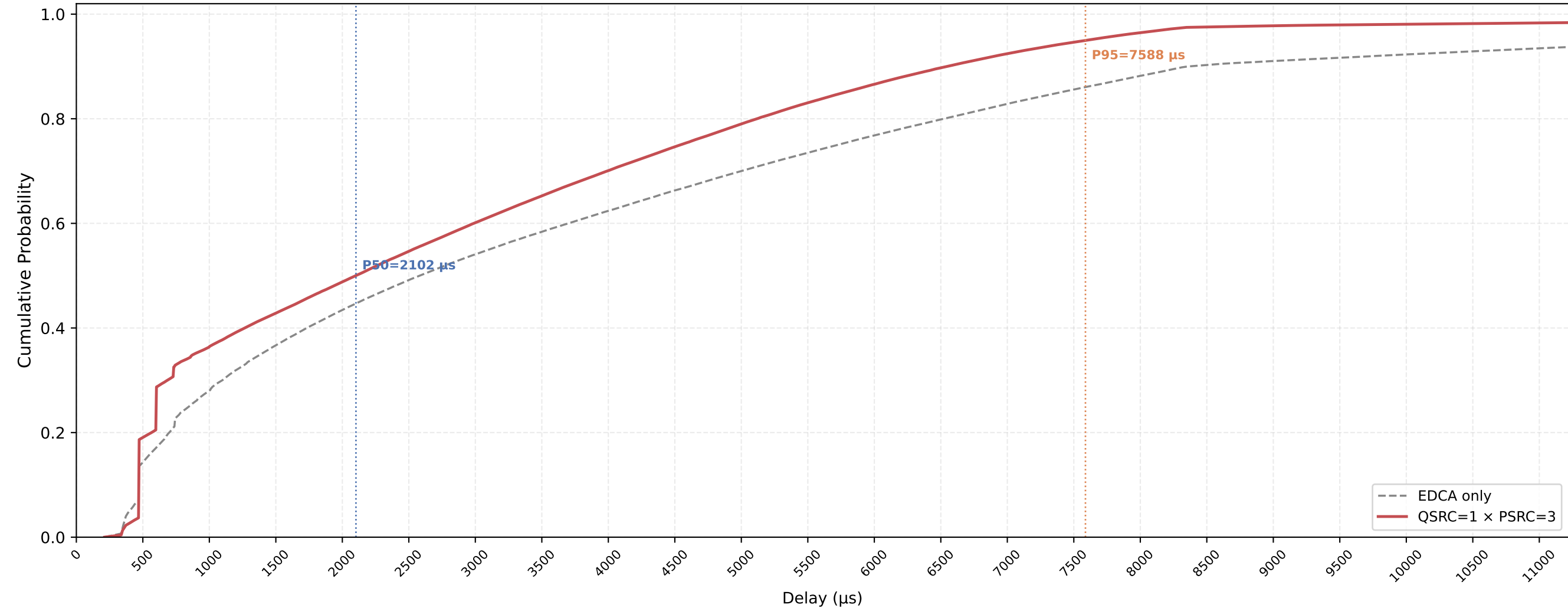
VO (all STAs) Delay CDF — QSRC=1 × PSRC=3 nSta=30, nPedca=30, 1Mbps, avg of 10 runs
