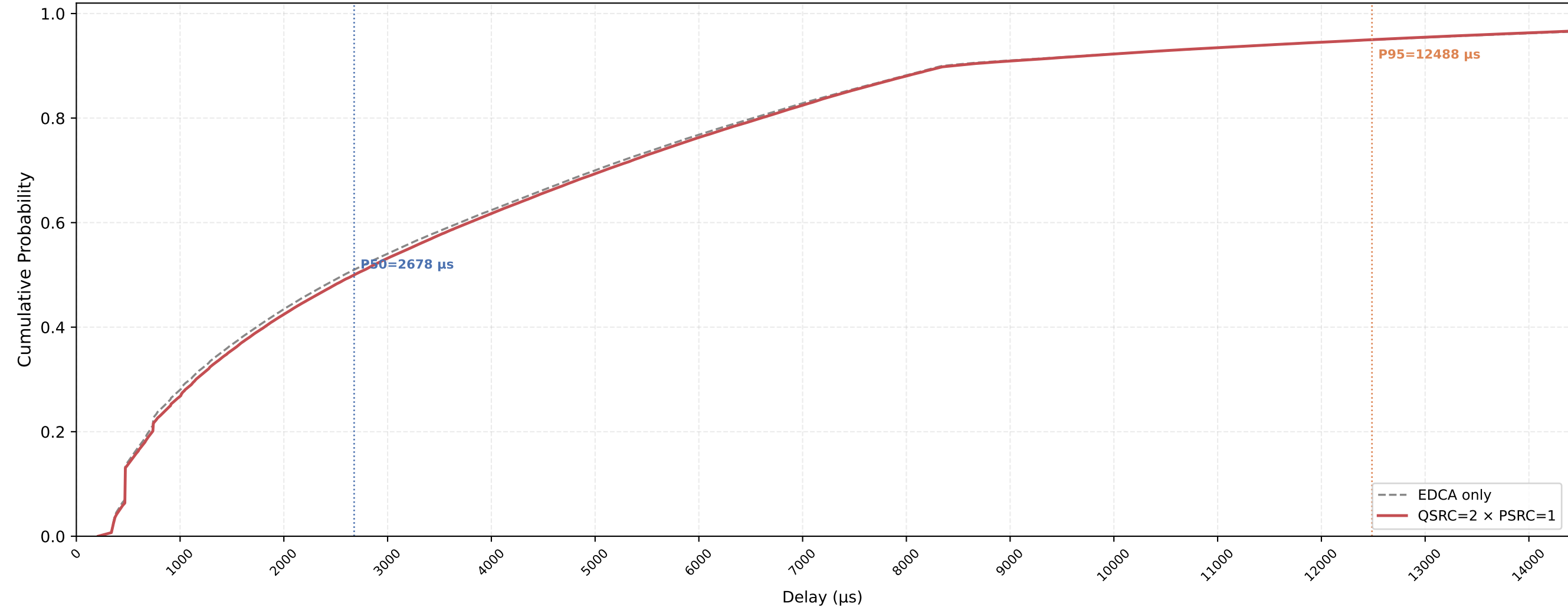
Legacy STA VO Delay CDF — QSRC=2 × PSRC=1 nSta=30, nPedca=5, 1Mbps, avg of 10 runs
