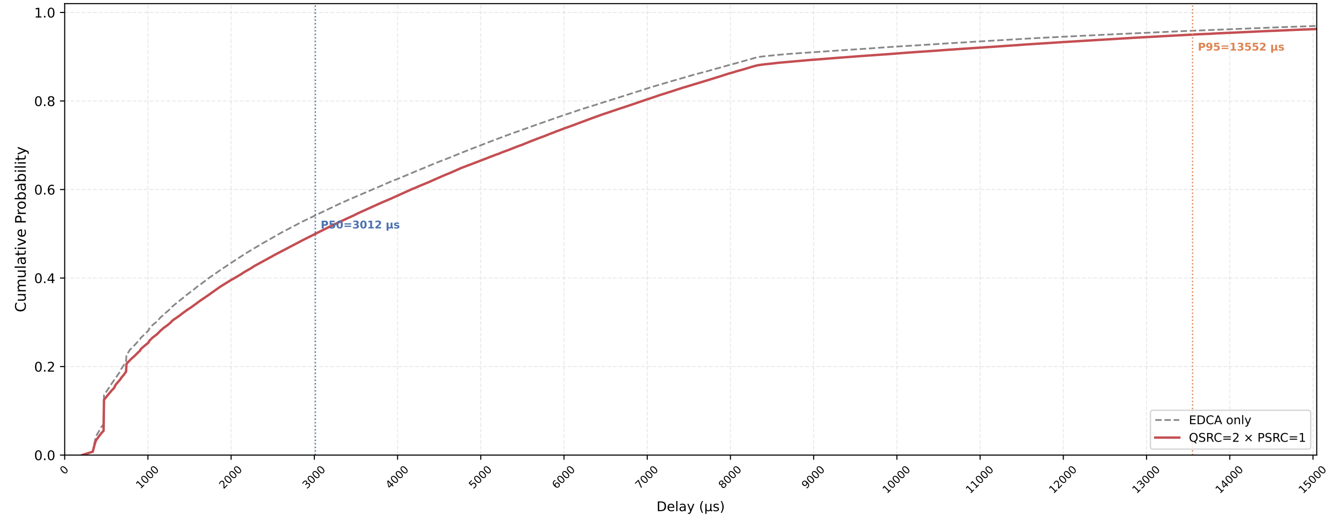
Legacy STA VO Delay CDF — QSRC=2 × PSRC=1 nSta=30, nPedca=15, 1Mbps, avg of 10 runs
