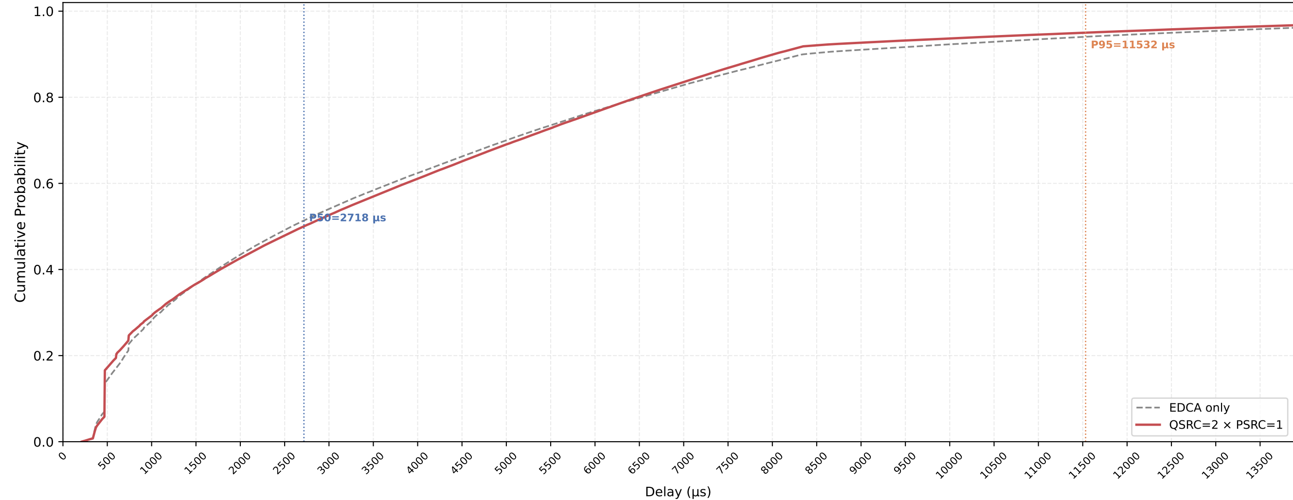
VO (all STAs) Delay CDF — QSRC=2 × PSRC=1 nSta=30, nPedca=15, 1Mbps, avg of 10 runs
