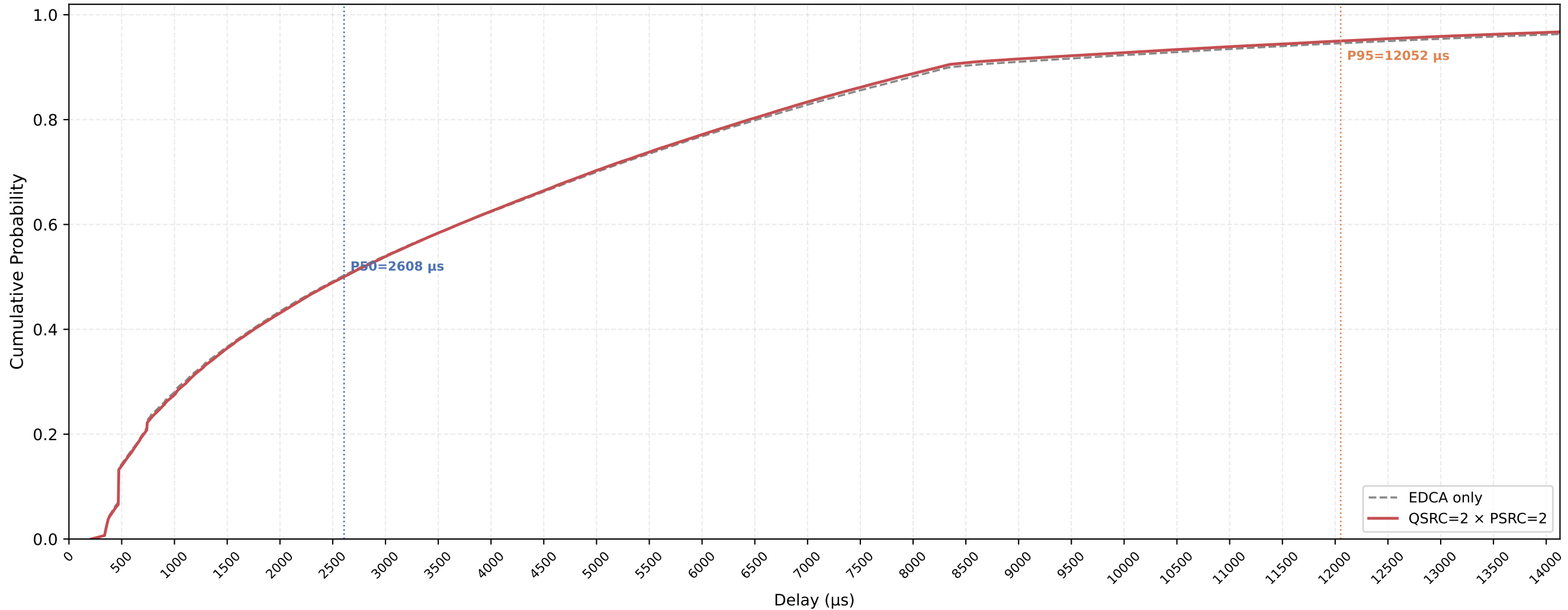
Legacy STA VO Delay CDF — QSRC=2 × PSRC=2 nSta=30, nPedca=5, 1Mbps, avg of 10 runs
