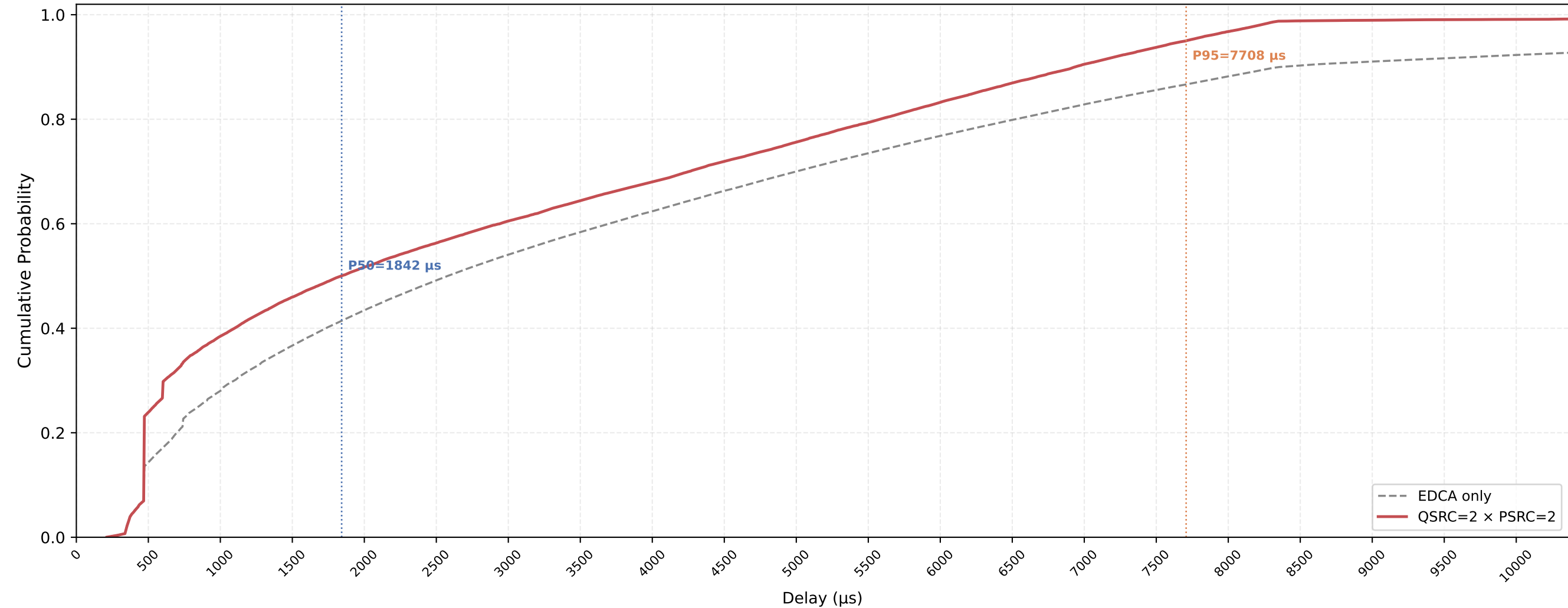
P-EDCA STA VO Delay CDF — QSRC=2 × PSRC=2 nSta=30, nPedca=5, 1Mbps, avg of 10 runs
