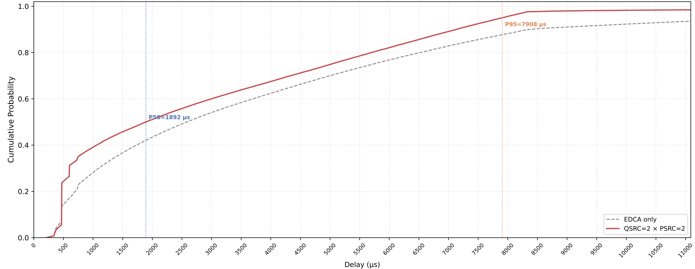
P-EDCA STA VO Delay CDF — QSRC=2 × PSRC=2 nSta=30, nPedca=15, 1Mbps, avg of 10 runs
