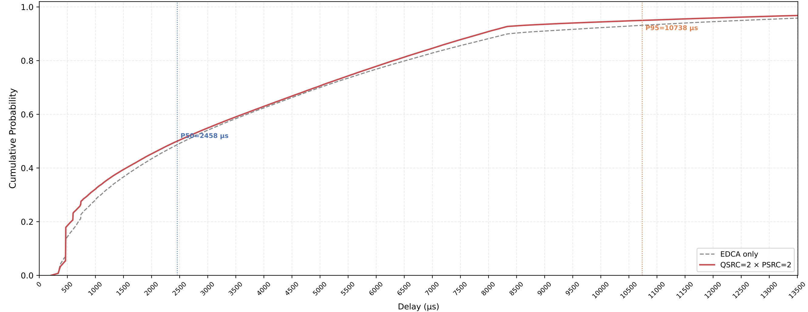
VO (all STAs) Delay CDF — QSRC=2 × PSRC=2 nSta=30, nPedca=15, 1Mbps, avg of 10 runs
