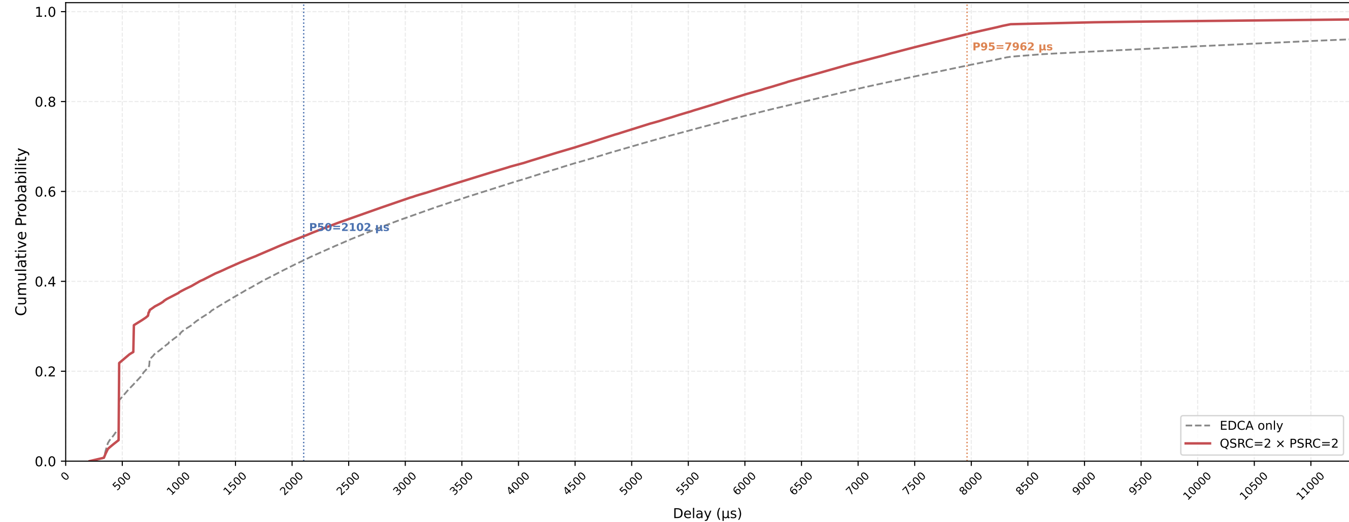
VO (all STAs) Delay CDF — QSRC=2 × PSRC=2 nSta=30, nPedca=30, 1Mbps, avg of 10 runs
