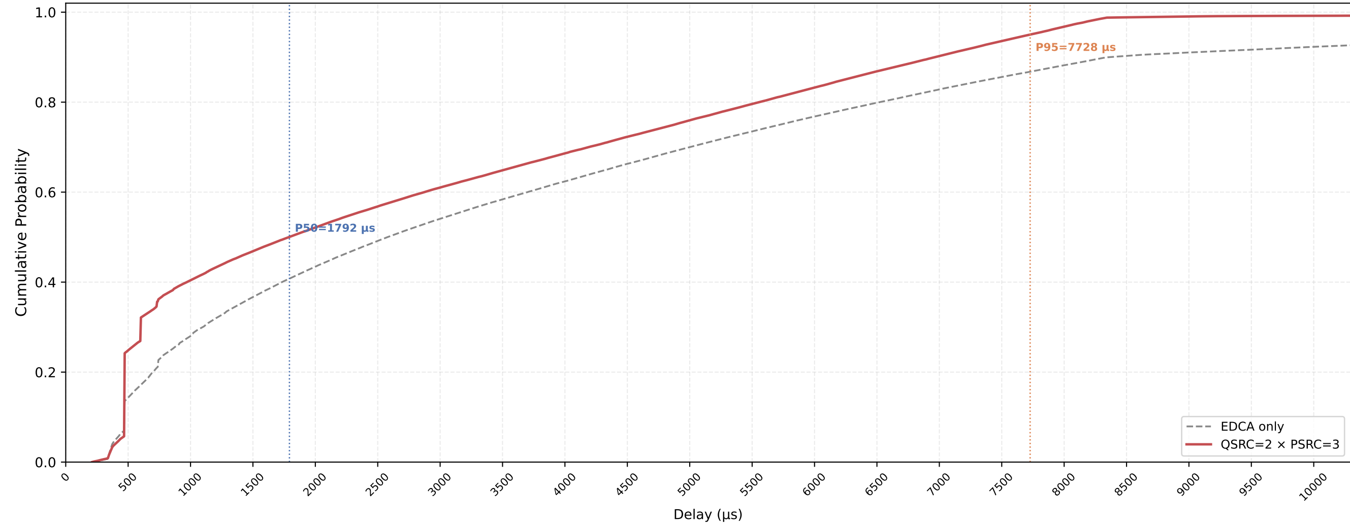
P-EDCA STA VO Delay CDF — QSRC=2 × PSRC=3 nSta=30, nPedca=15, 1Mbps, avg of 10 runs
