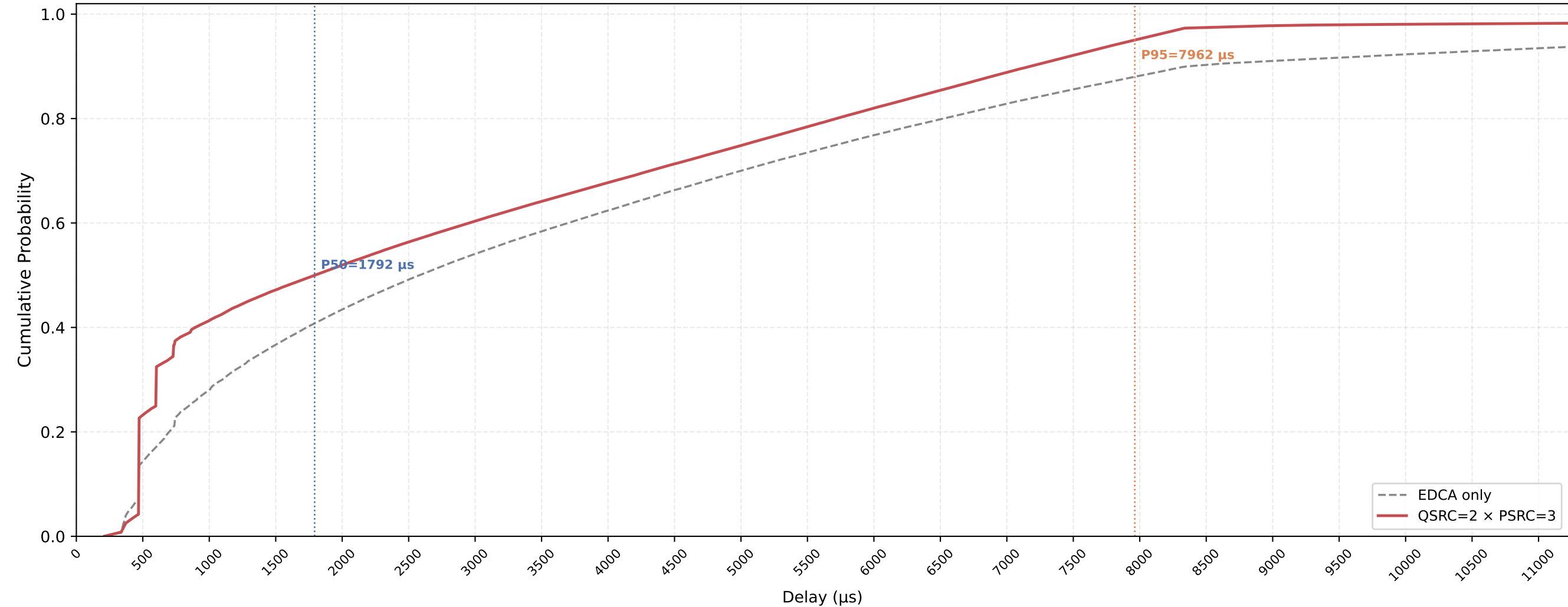
P-EDCA STA VO Delay CDF — QSRC=2 × PSRC=3 nSta=30, nPedca=30, 1Mbps, avg of 10 runs
