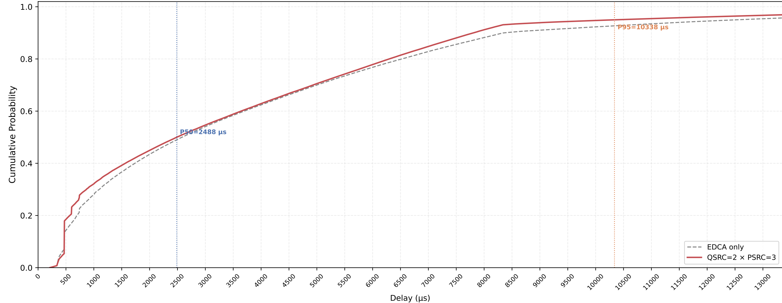
VO (all STAs) Delay CDF — QSRC=2 × PSRC=3 nSta=30, nPedca=15, 1Mbps, avg of 10 runs
