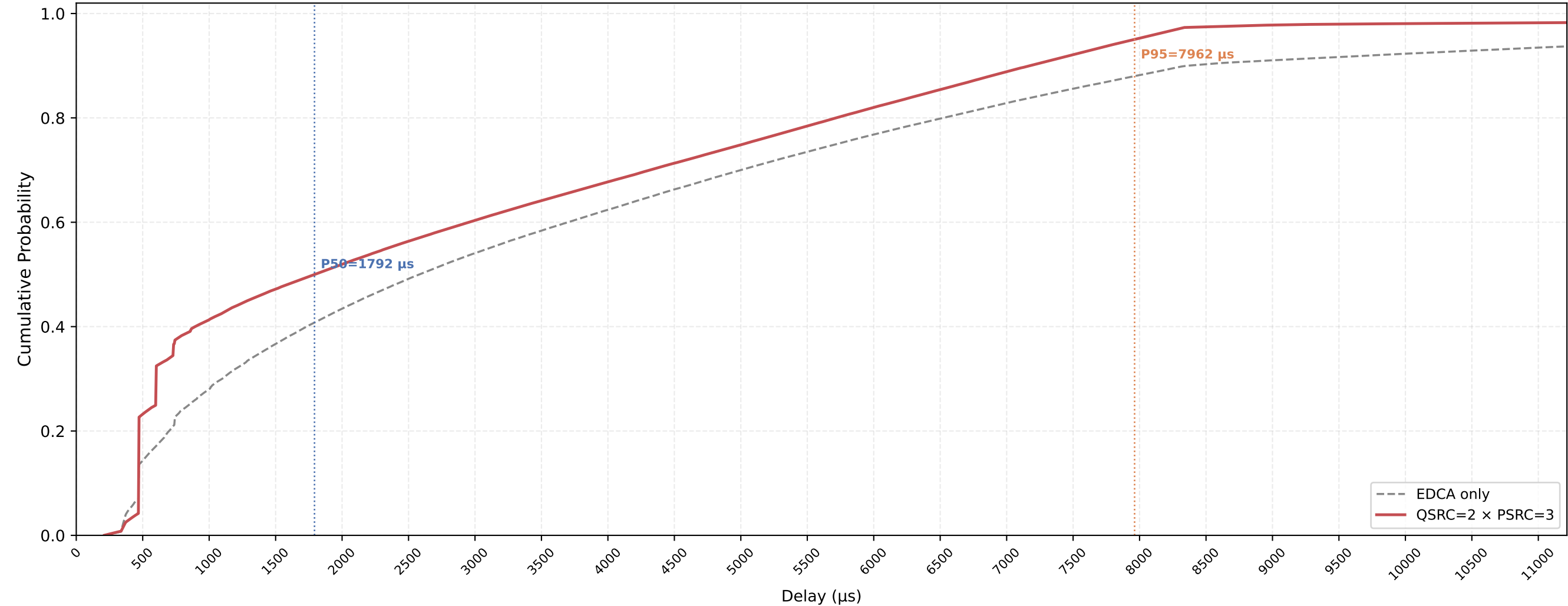
VO (all STAs) Delay CDF — QSRC=2 × PSRC=3 nSta=30, nPedca=30, 1Mbps, avg of 10 runs
