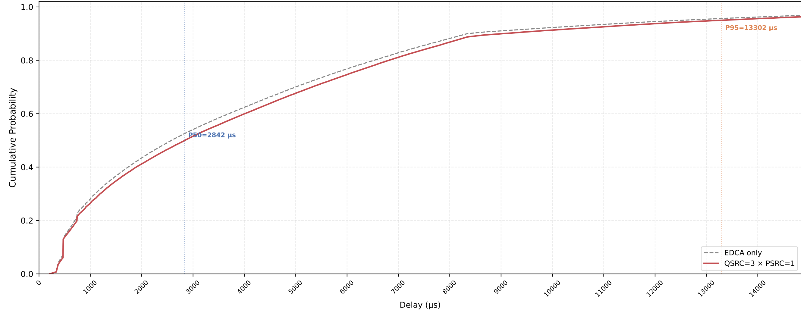
Legacy STA VO Delay CDF — QSRC=3 × PSRC=1 nSta=30, nPedca=15, 1Mbps, avg of 10 runs
