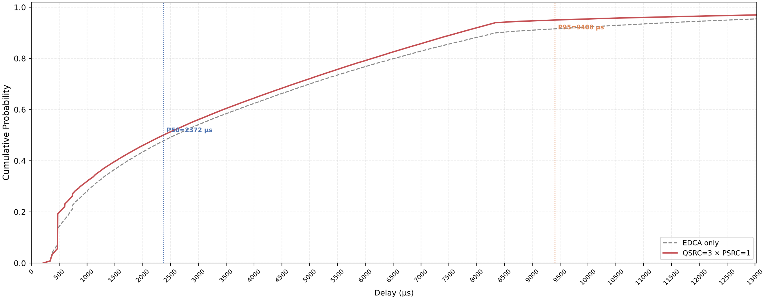
P-EDCA STA VO Delay CDF — QSRC=3 × PSRC=1 nSta=30, nPedca=30, 1Mbps, avg of 10 runs
