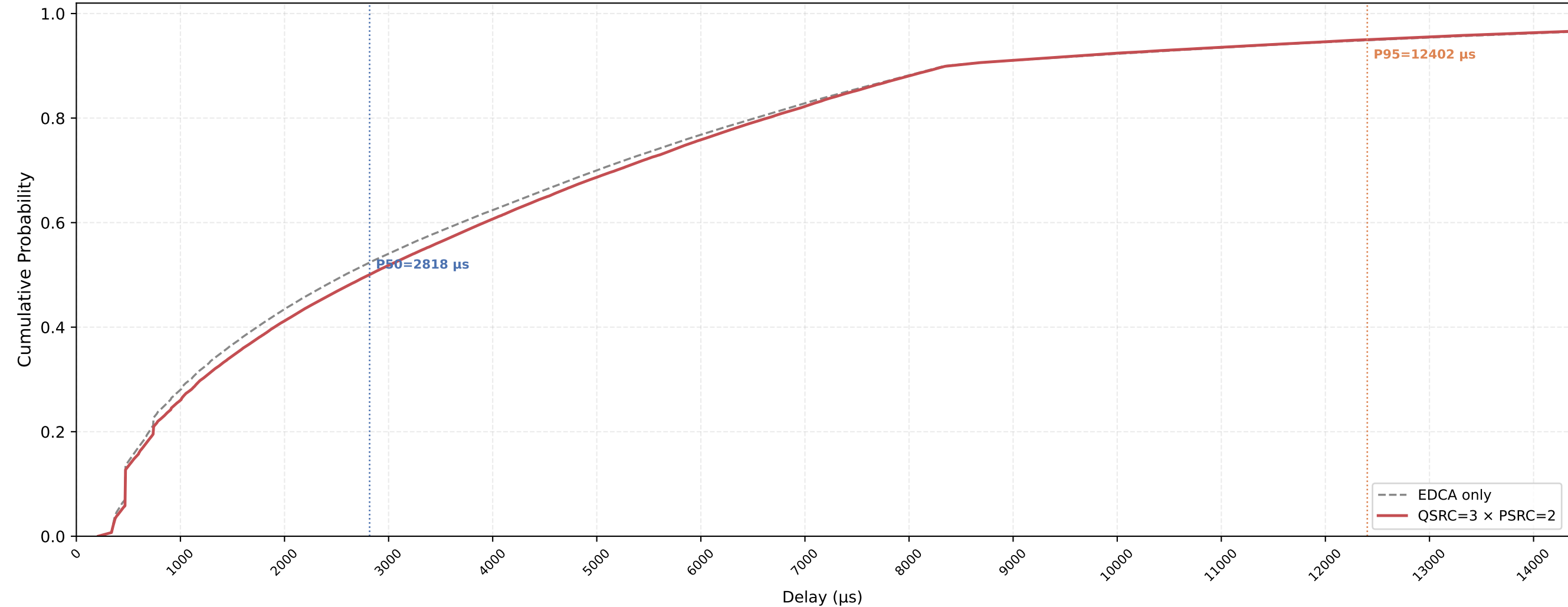
Legacy STA VO Delay CDF — QSRC=3 × PSRC=2 nSta=30, nPedca=15, 1Mbps, avg of 10 runs
