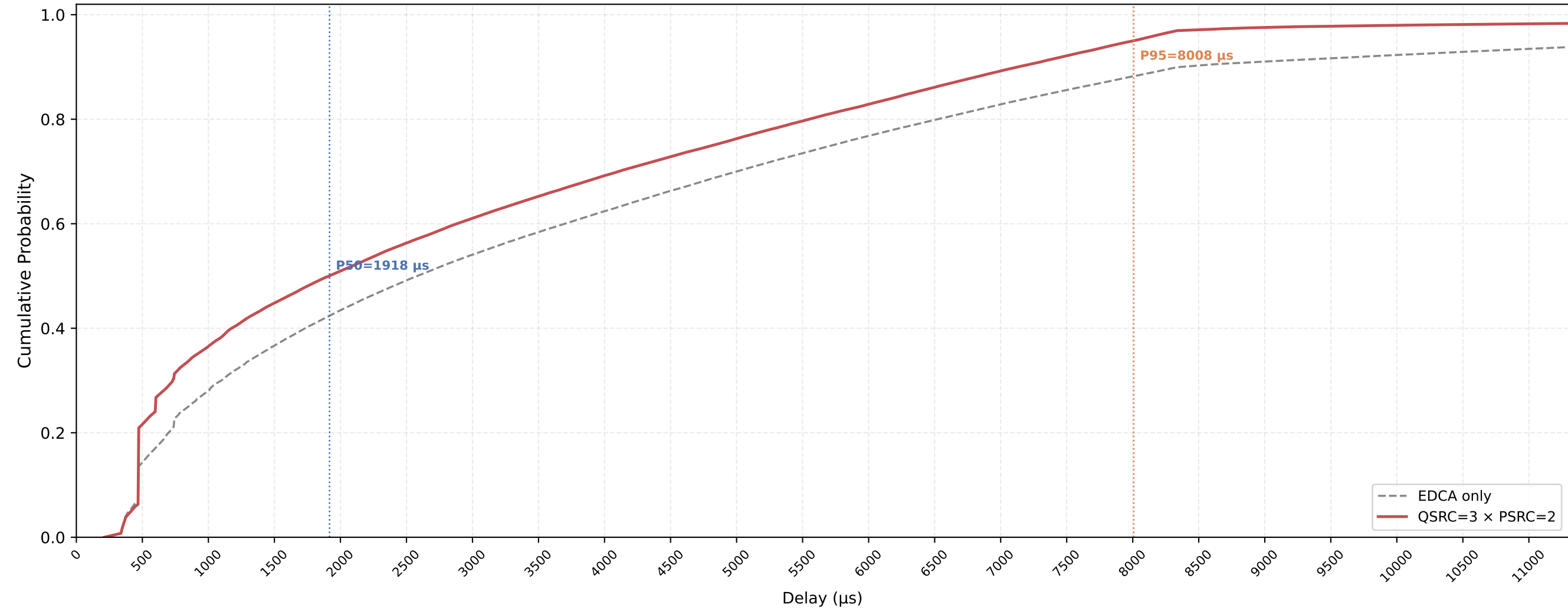
P-EDCA STA VO Delay CDF — QSRC=3 × PSRC=2 nSta=30, nPedca=15, 1Mbps, avg of 10 runs
