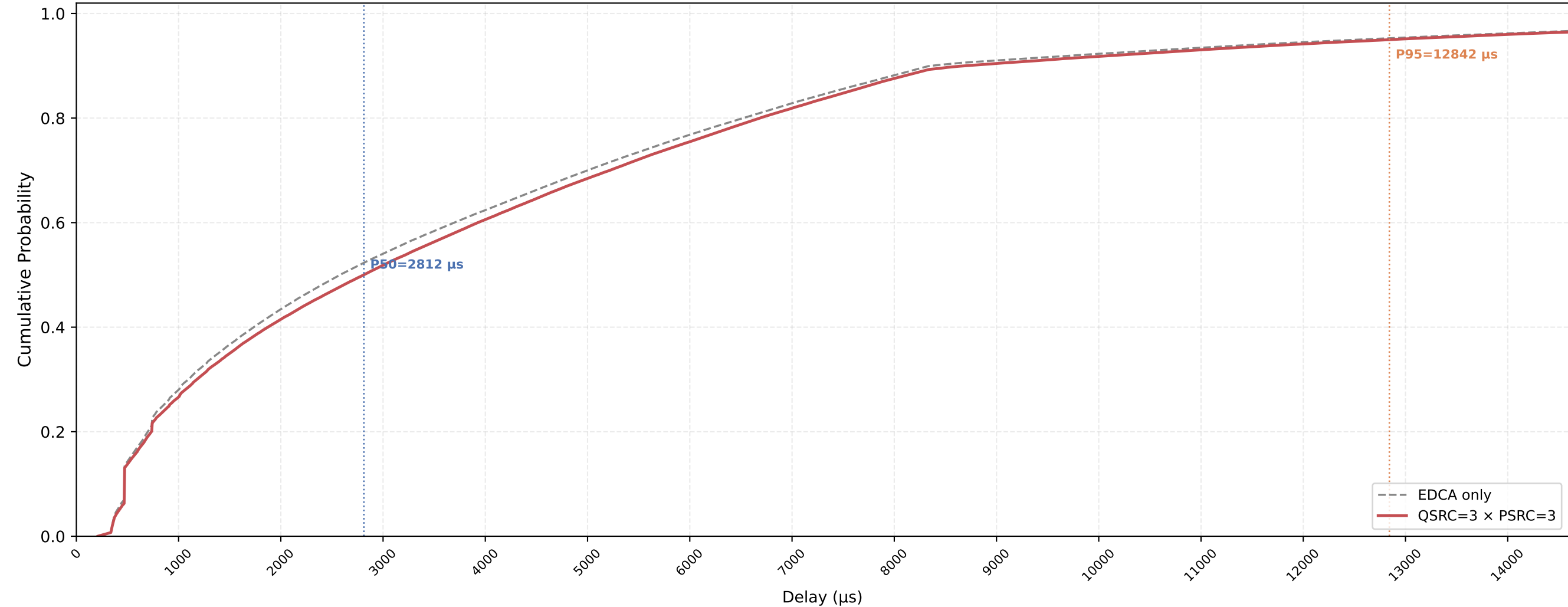
Legacy STA VO Delay CDF — QSRC=3 × PSRC=3 nSta=30, nPedca=5, 1Mbps, avg of 10 runs
