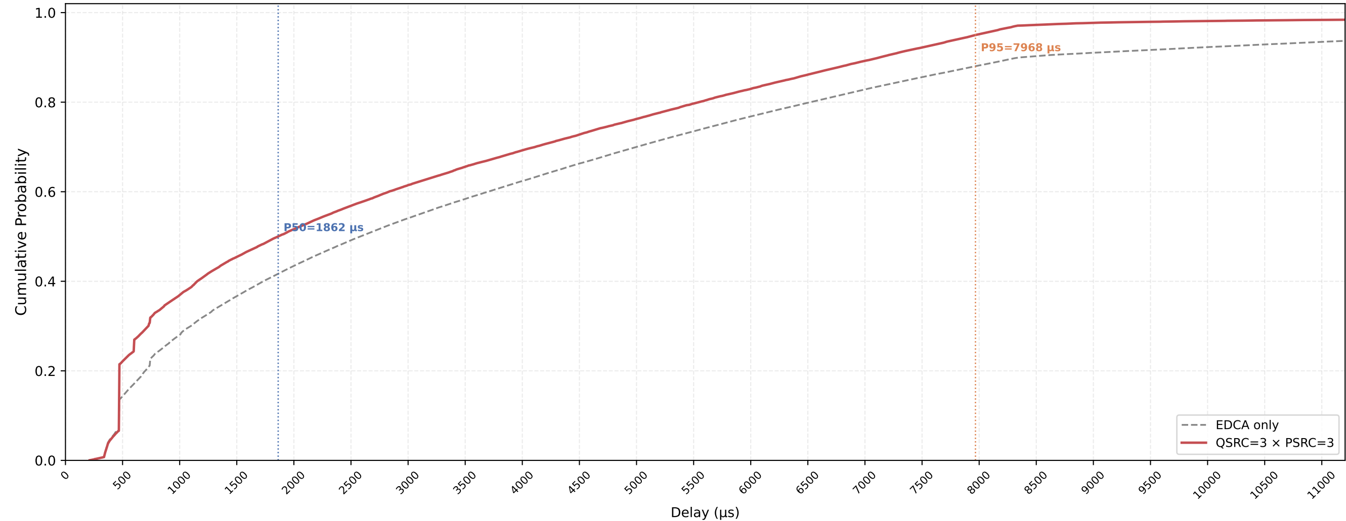
P-EDCA STA VO Delay CDF — QSRC=3 × PSRC=3 nSta=30, nPedca=5, 1Mbps, avg of 10 runs
