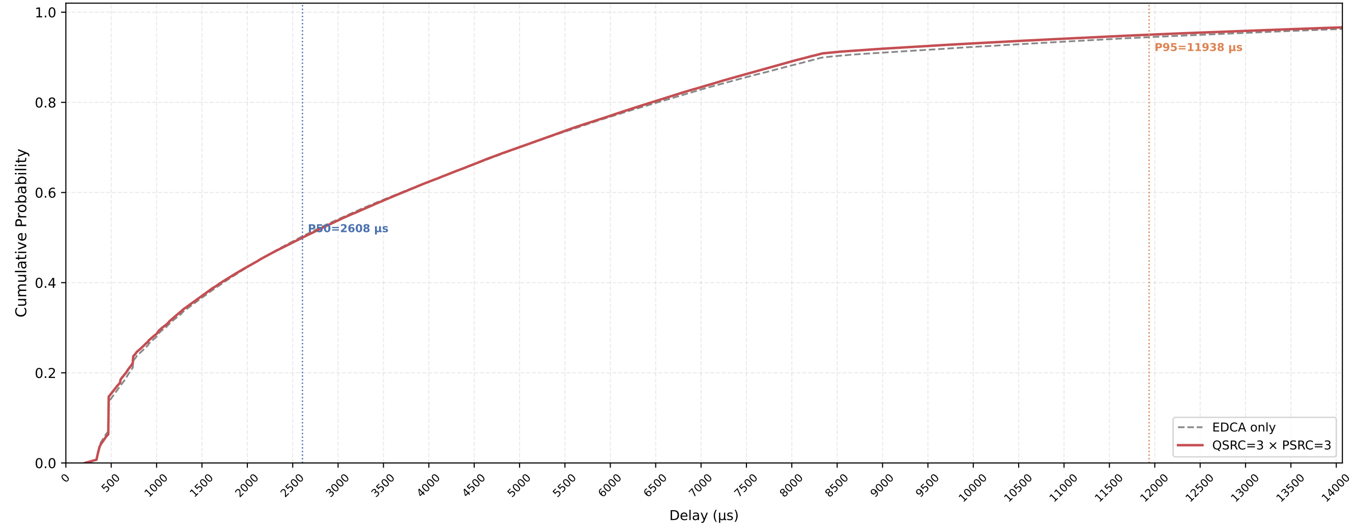
VO (all STAs) Delay CDF — QSRC=3 × PSRC=3 nSta=30, nPedca=5, 1Mbps, avg of 10 runs
