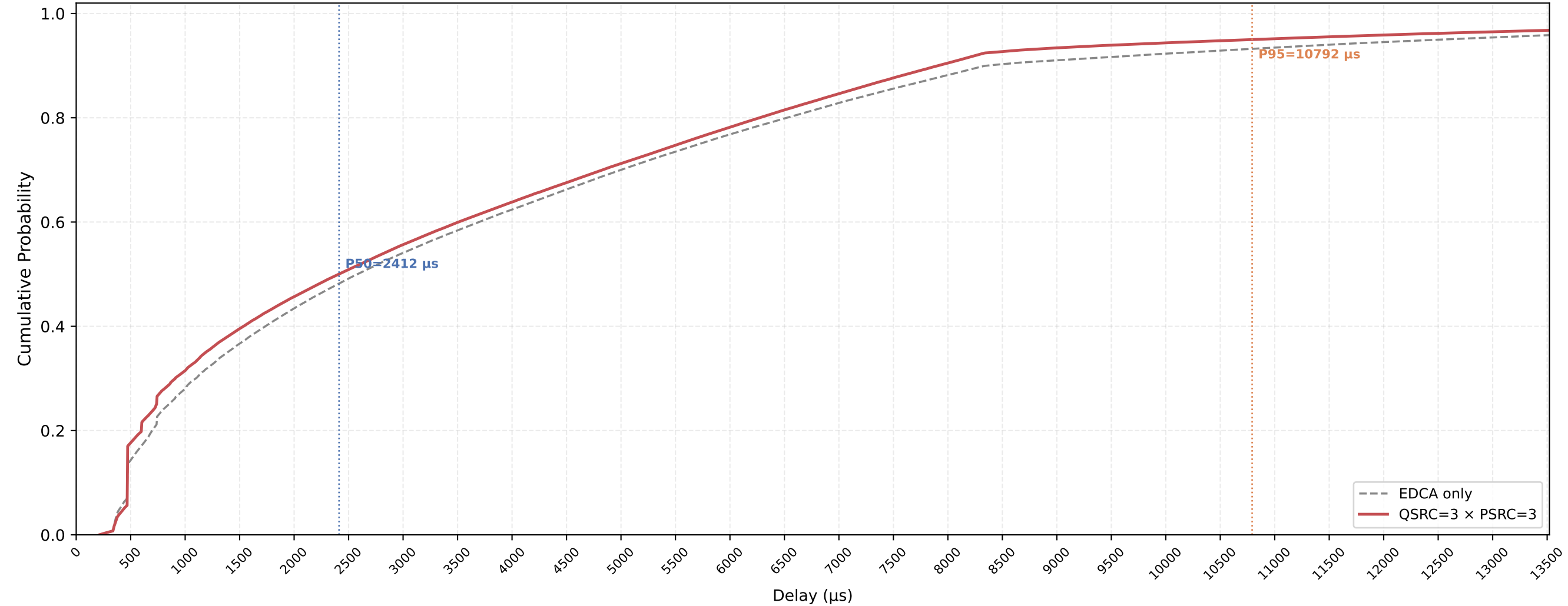
VO (all STAs) Delay CDF — QSRC=3 × PSRC=3 nSta=30, nPedca=15, 1Mbps, avg of 10 runs
