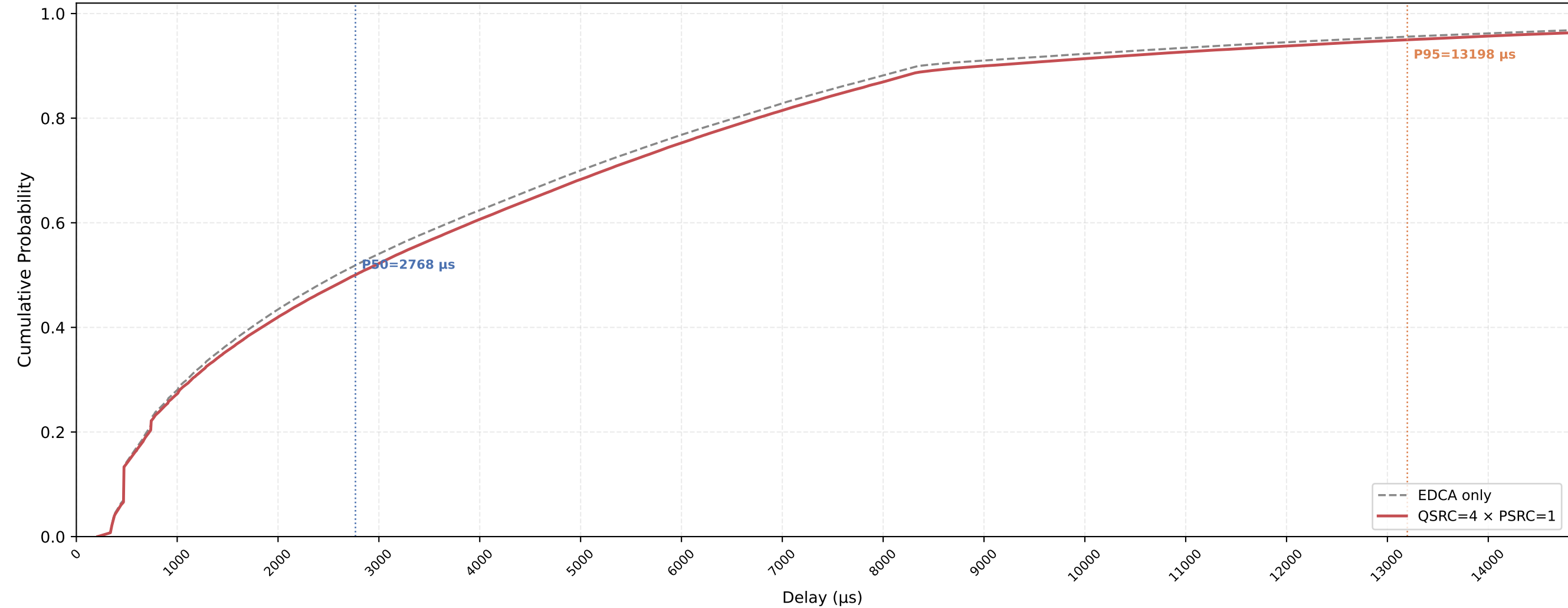
Legacy STA VO Delay CDF — QSRC=4 × PSRC=1 nSta=30, nPedca=5, 1Mbps, avg of 10 runs
