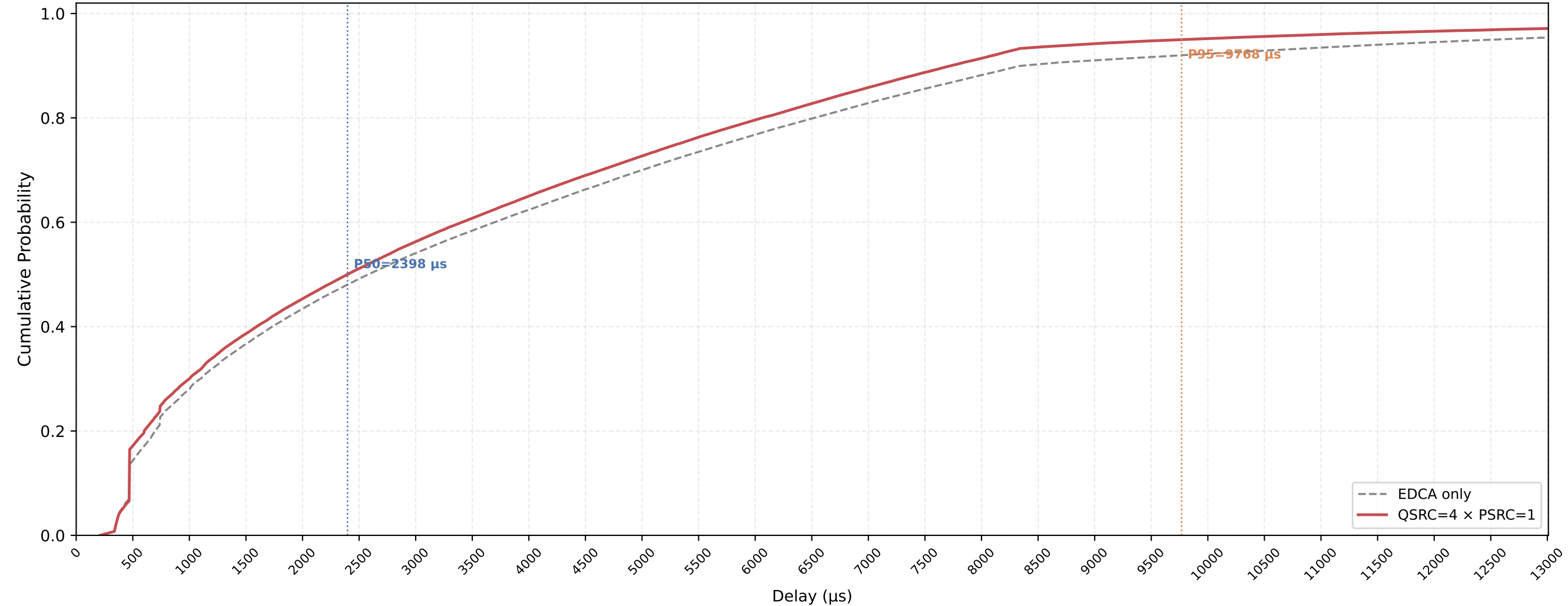
P-EDCA STA VO Delay CDF — QSRC=4 × PSRC=1 nSta=30, nPedca=15, 1Mbps, avg of 10 runs
