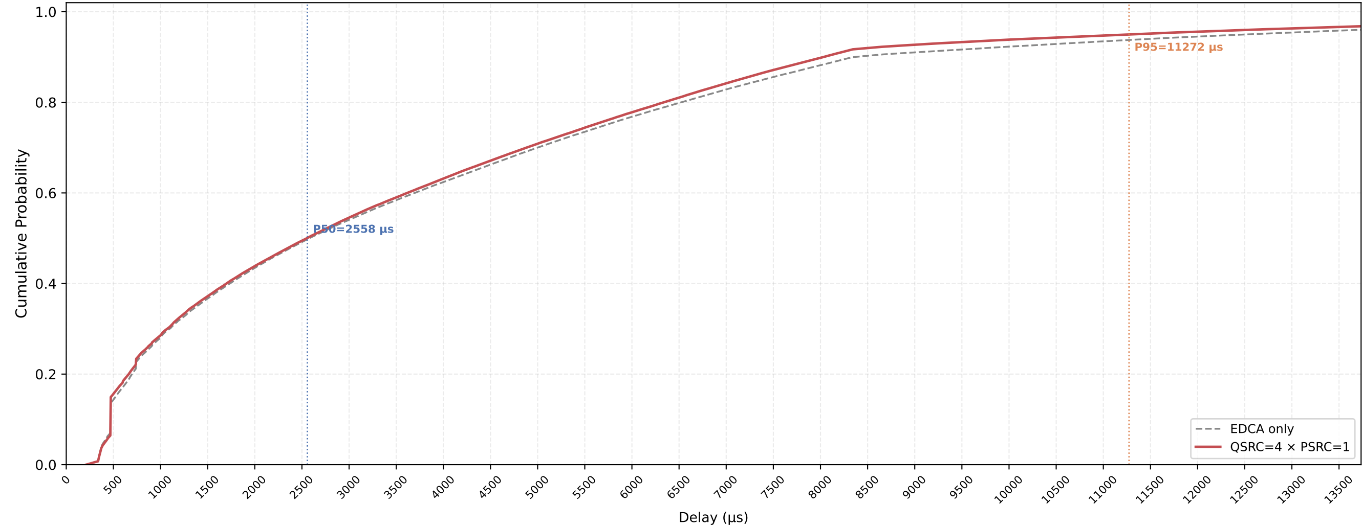
VO (all STAs) Delay CDF — QSRC=4 × PSRC=1 nSta=30, nPedca=15, 1Mbps, avg of 10 runs
