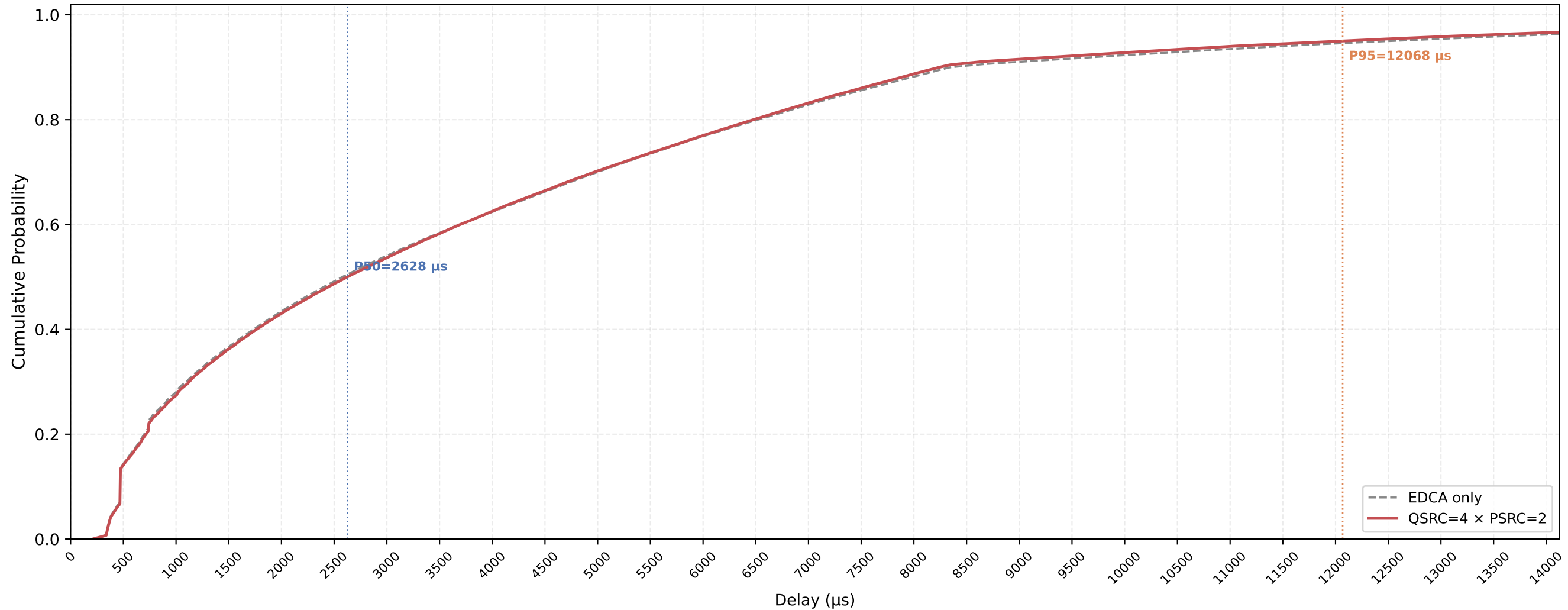
Legacy STA VO Delay CDF — QSRC=4 × PSRC=2 nSta=30, nPedca=5, 1Mbps, avg of 10 runs
