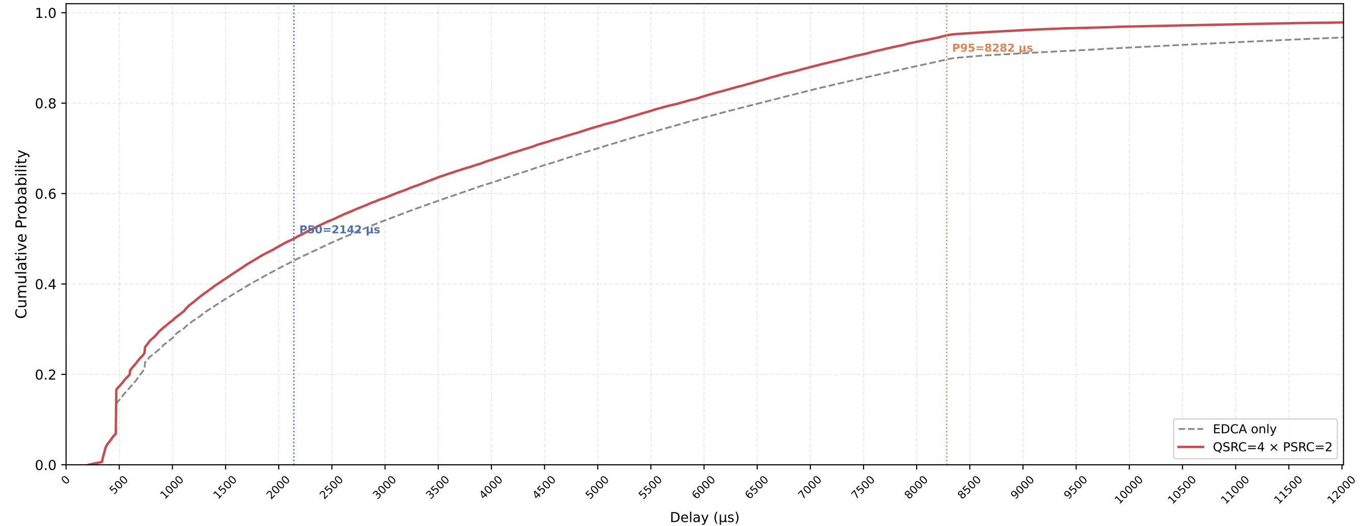
P-EDCA STA VO Delay CDF — QSRC=4 × PSRC=2 nSta=30, nPedca=5, 1Mbps, avg of 10 runs
