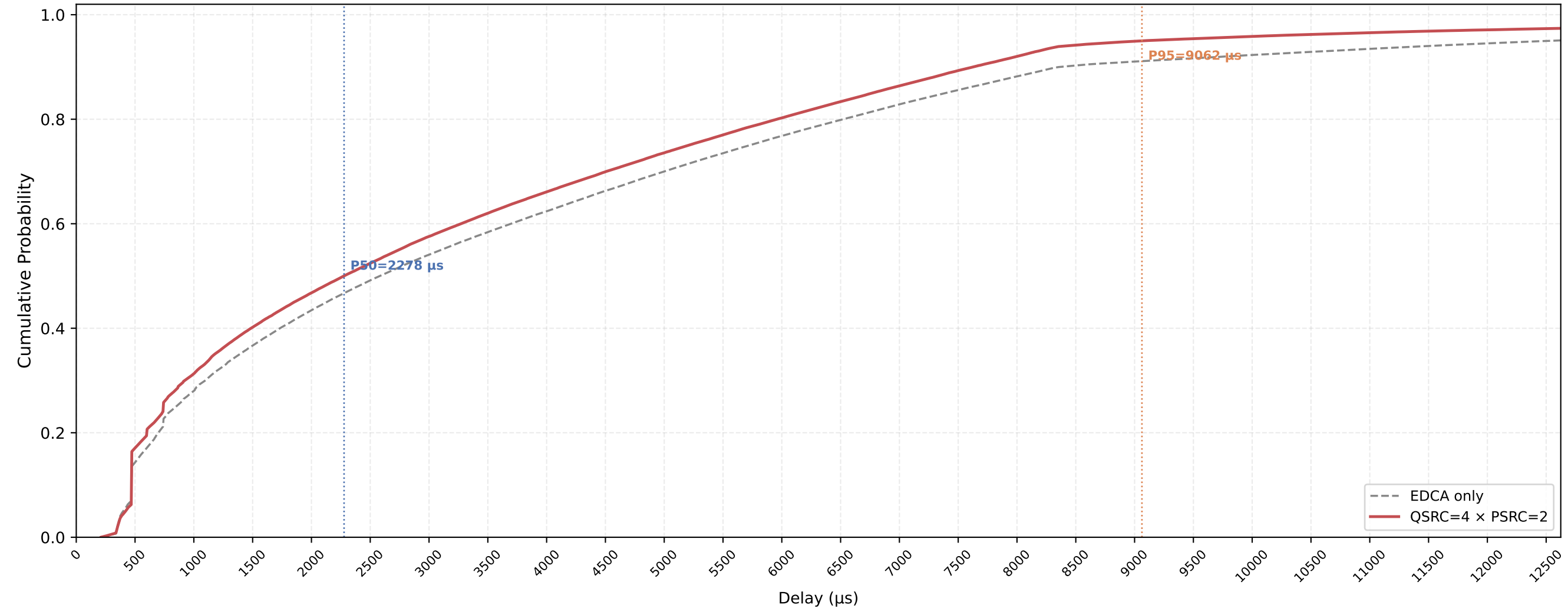
P-EDCA STA VO Delay CDF — QSRC=4 × PSRC=2 nSta=30, nPedca=15, 1Mbps, avg of 10 runs
