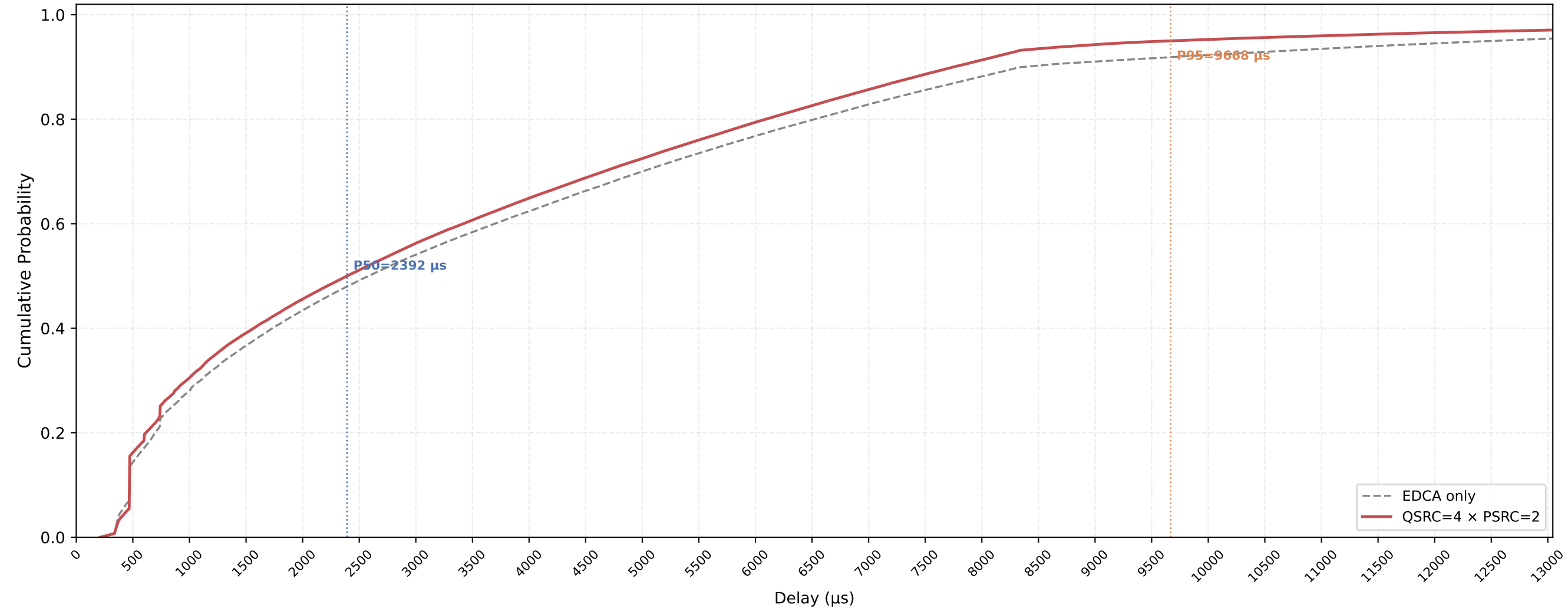
P-EDCA STA VO Delay CDF — QSRC=4 × PSRC=2 nSta=30, nPedca=30, 1Mbps, avg of 10 runs
