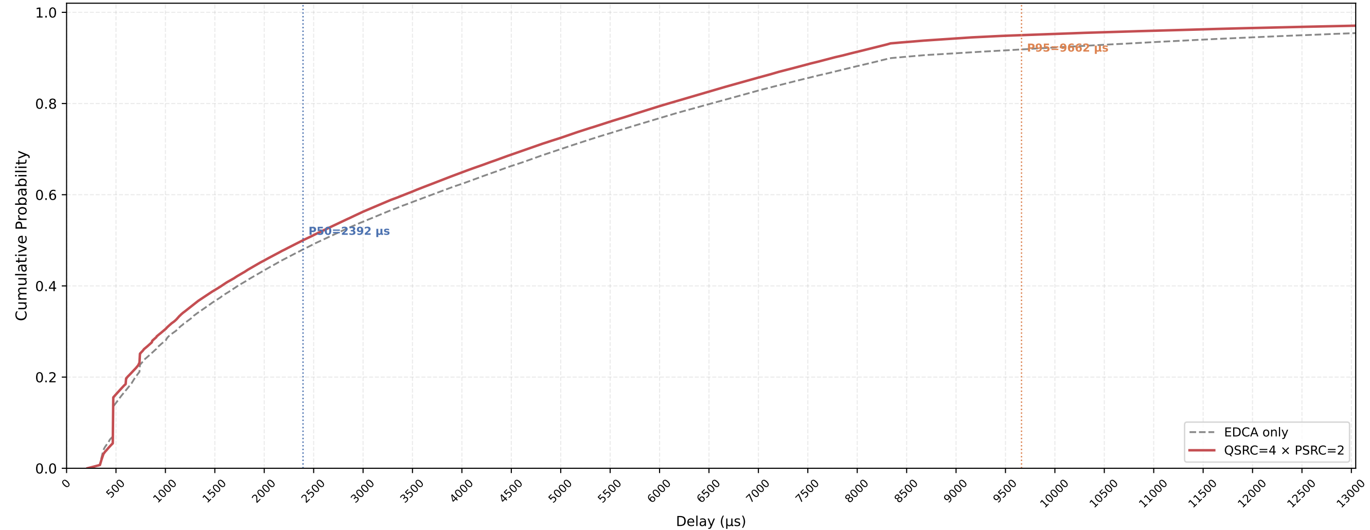
VO (all STAs) Delay CDF — QSRC=4 × PSRC=2 nSta=30, nPedca=30, 1Mbps, avg of 10 runs
