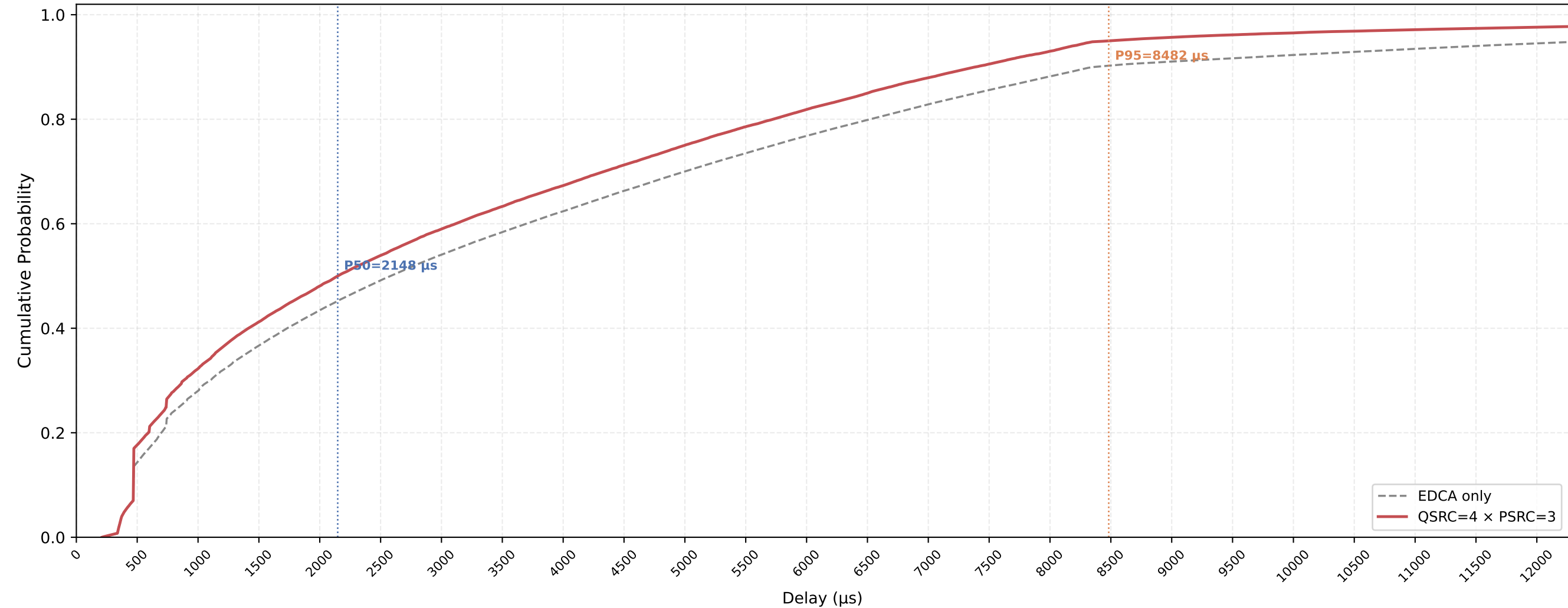
P-EDCA STA VO Delay CDF — QSRC=4 × PSRC=3 nSta=30, nPedca=5, 1Mbps, avg of 10 runs
