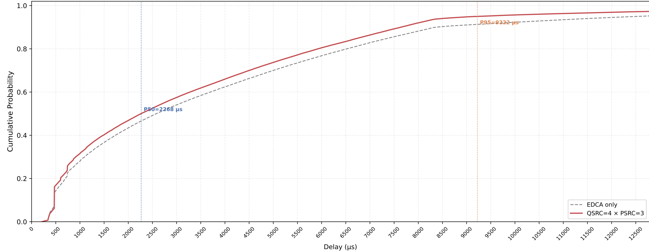
P-EDCA STA VO Delay CDF — QSRC=4 × PSRC=3 nSta=30, nPedca=15, 1Mbps, avg of 10 runs
