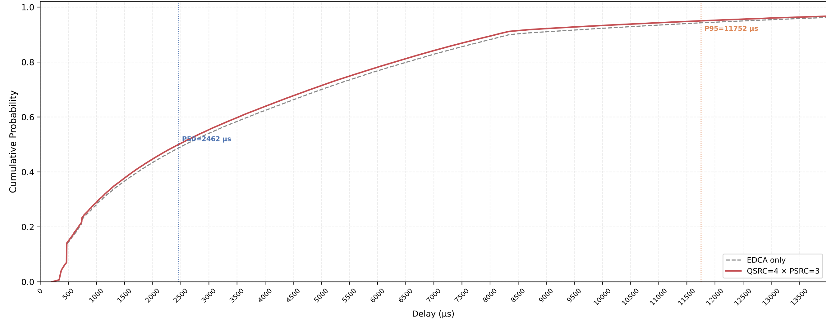
VO (all STAs) Delay CDF — QSRC=4 × PSRC=3 nSta=30, nPedca=5, 1Mbps, avg of 10 runs
