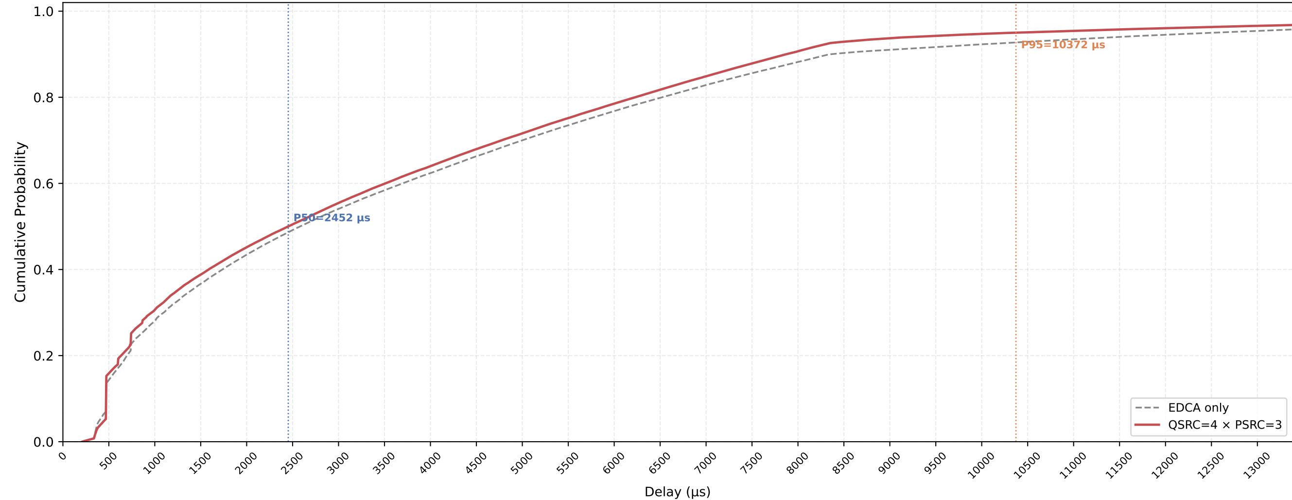
VO (all STAs) Delay CDF — QSRC=4 × PSRC=3 nSta=30, nPedca=30, 1Mbps, avg of 10 runs
