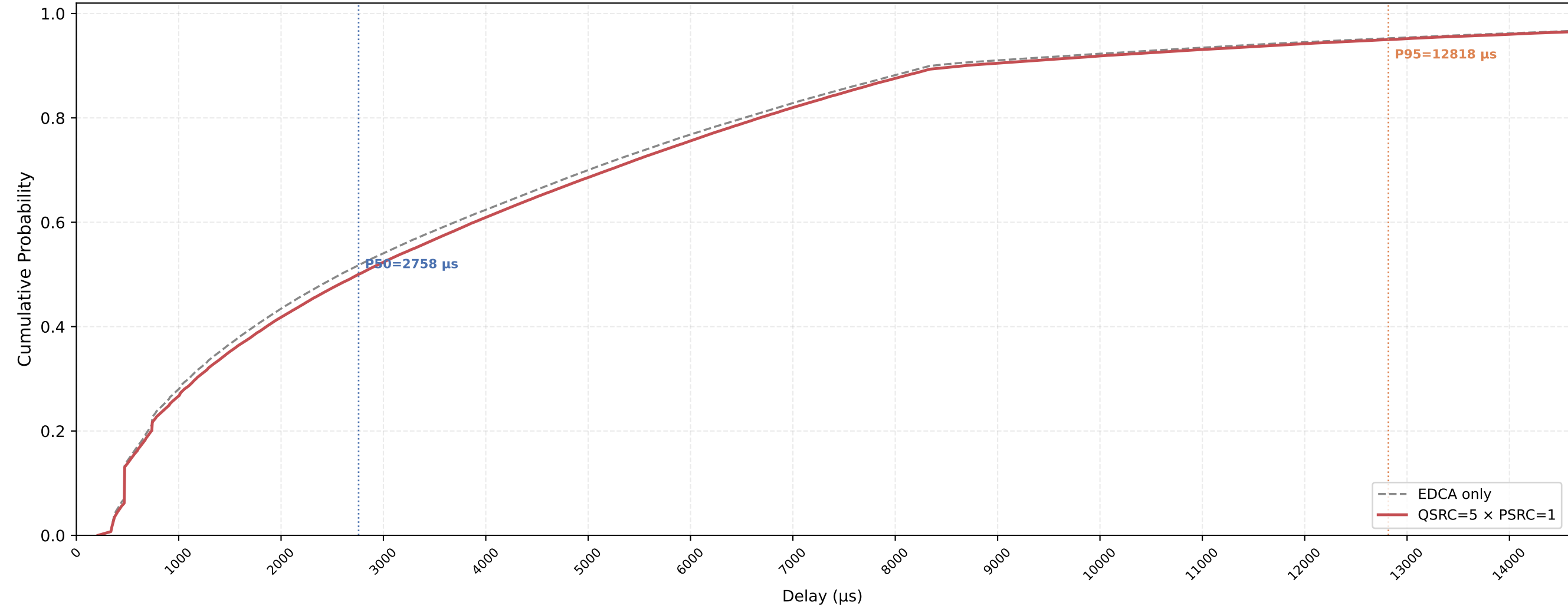
Legacy STA VO Delay CDF — QSRC=5 × PSRC=1 nSta=30, nPedca=15, 1Mbps, avg of 10 runs
