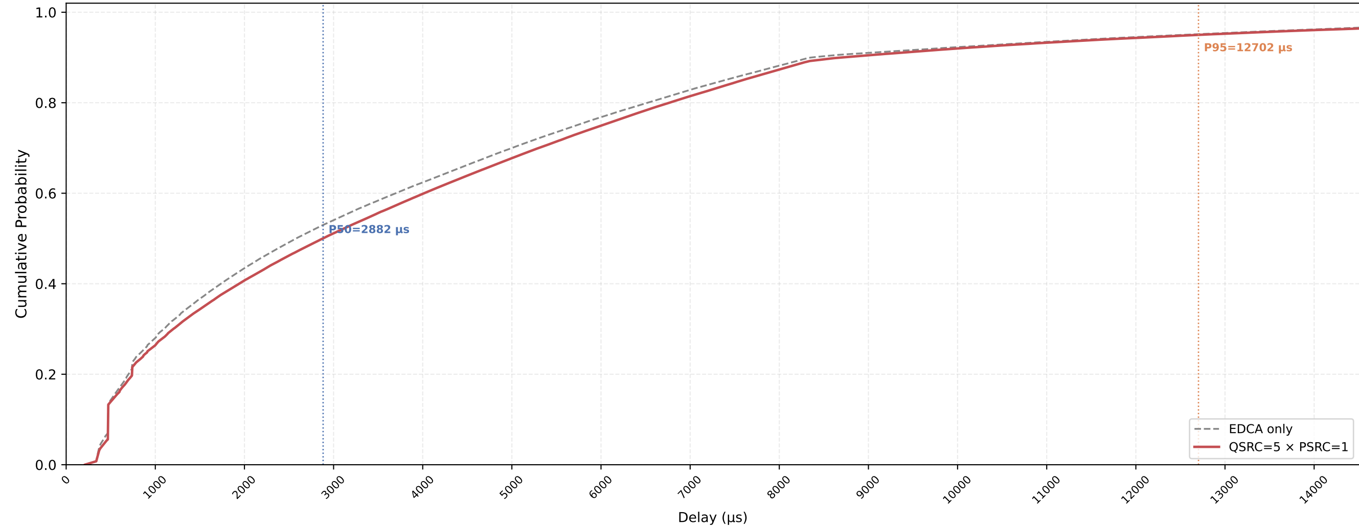
P-EDCA STA VO Delay CDF — QSRC=5 × PSRC=1 nSta=30, nPedca=30, 1Mbps, avg of 10 runs
