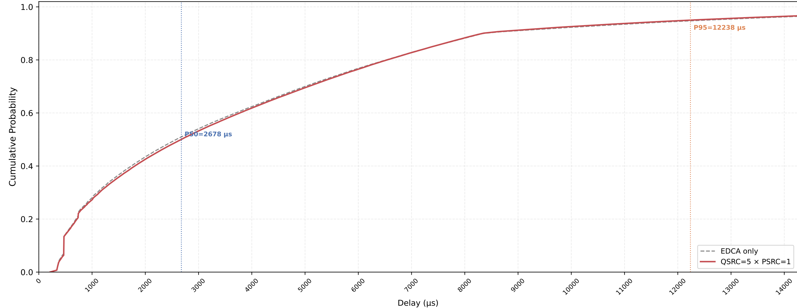
VO (all STAs) Delay CDF — QSRC=5 × PSRC=1 nSta=30, nPedca=15, 1Mbps, avg of 10 runs
