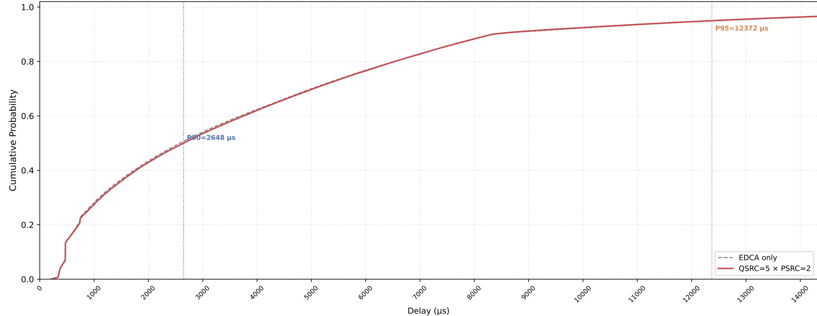
Legacy STA VO Delay CDF — QSRC=5 × PSRC=2 nSta=30, nPedca=5, 1Mbps, avg of 10 runs
