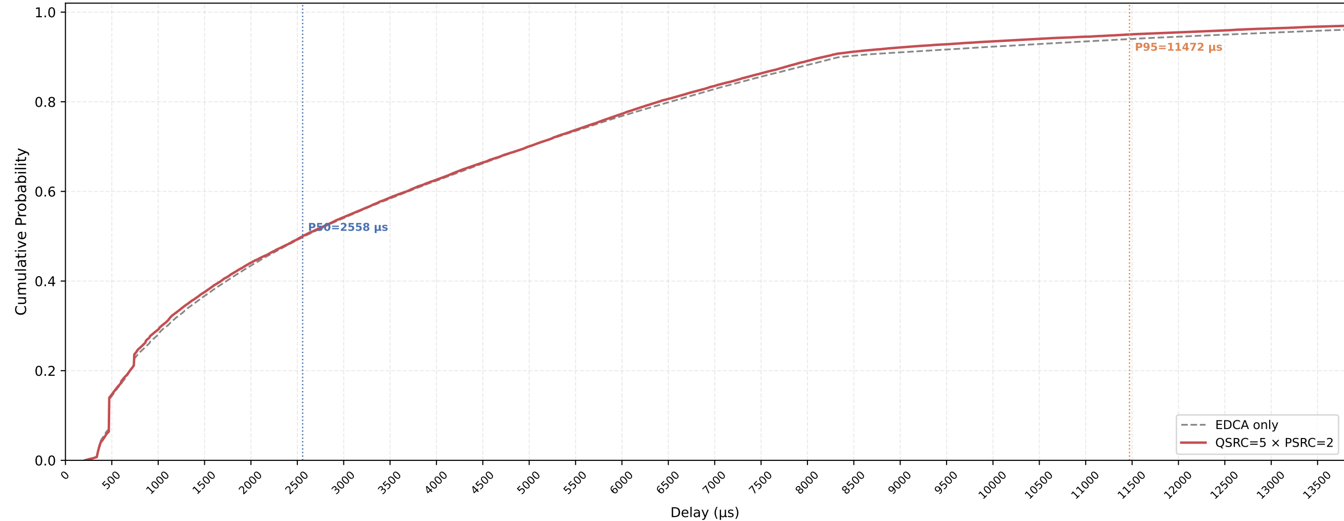
P-EDCA STA VO Delay CDF — QSRC=5 × PSRC=2 nSta=30, nPedca=5, 1Mbps, avg of 10 runs
