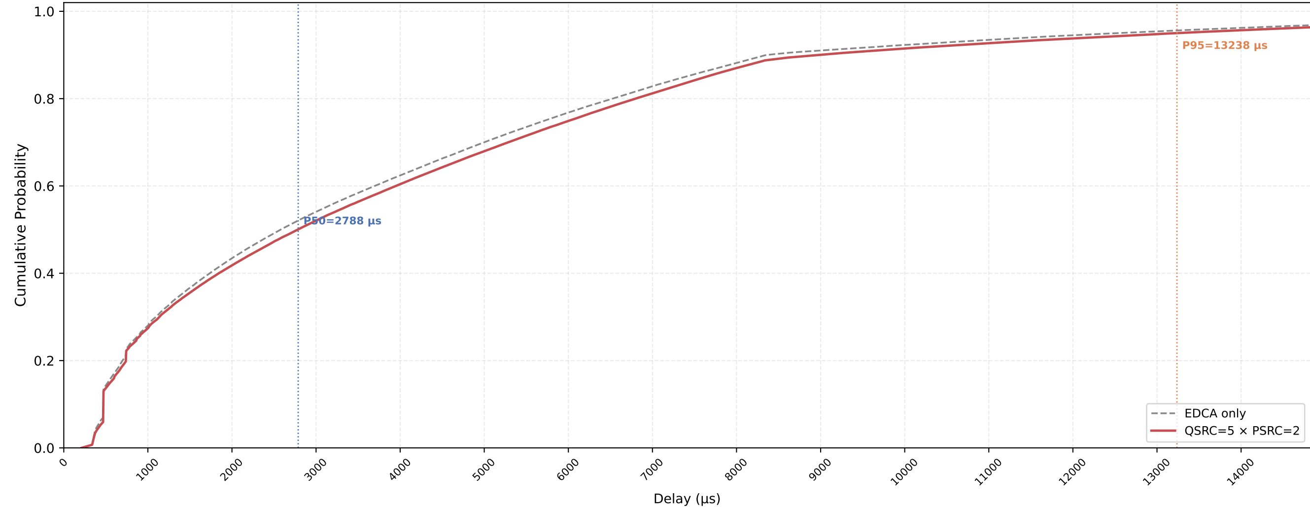
VO (all STAs) Delay CDF — QSRC=5 × PSRC=2 nSta=30, nPedca=15, 1Mbps, avg of 10 runs
