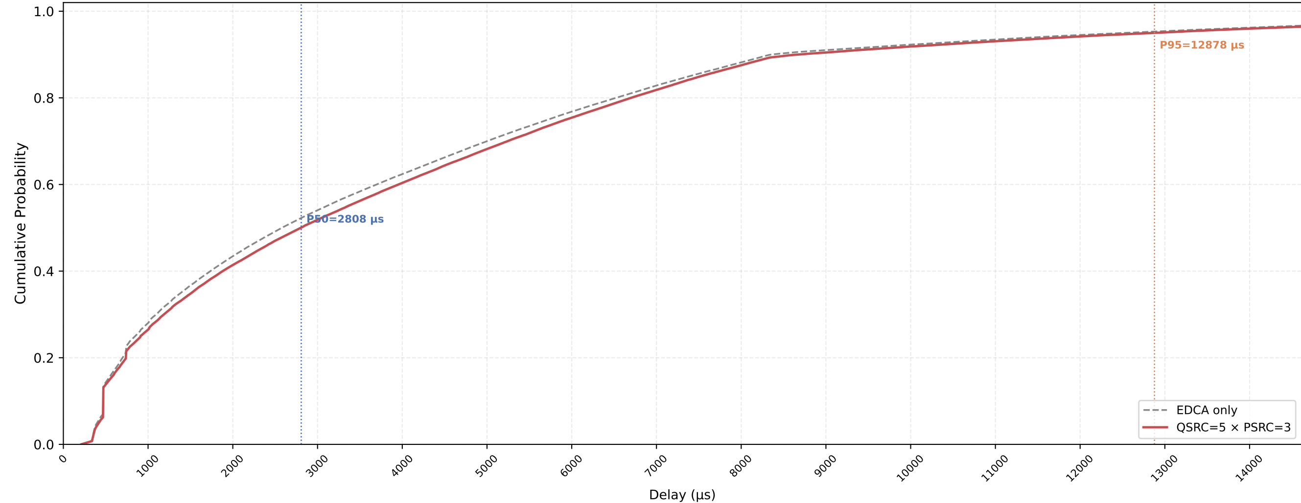
Legacy STA VO Delay CDF — QSRC=5 × PSRC=3 nSta=30, nPedca=15, 1Mbps, avg of 10 runs
