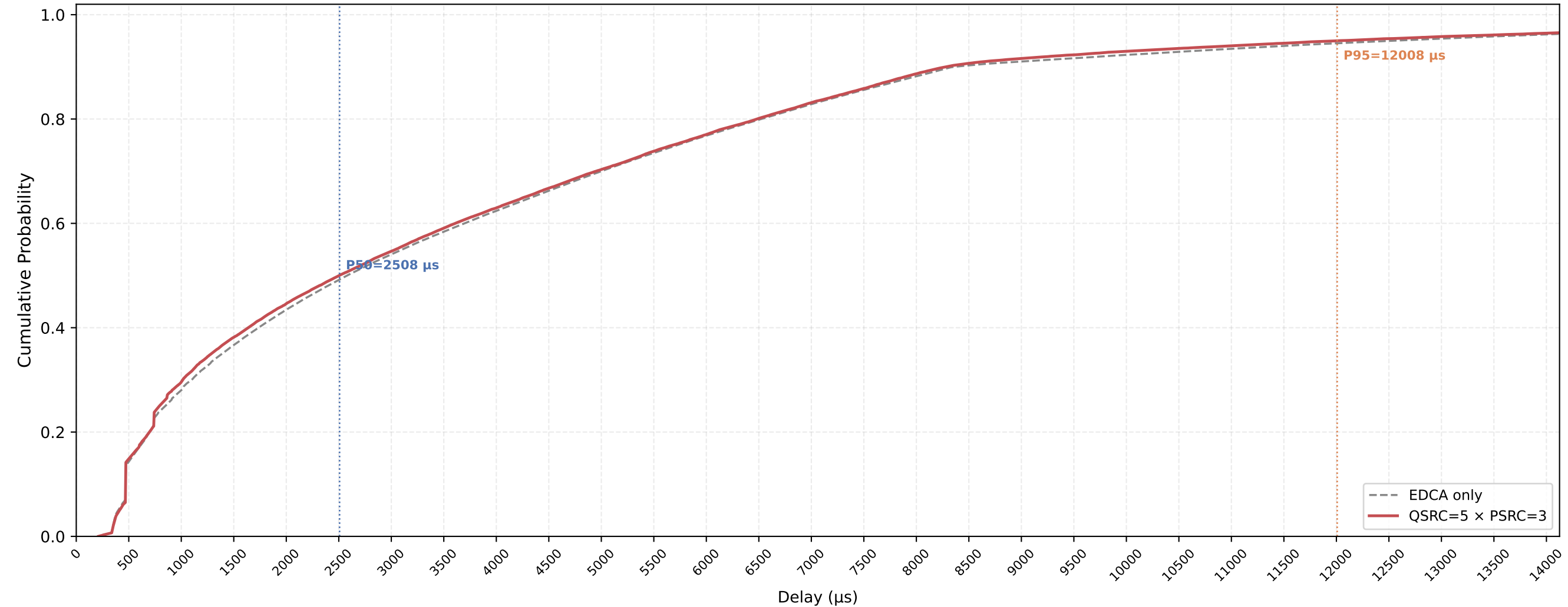
P-EDCA STA VO Delay CDF — QSRC=5 × PSRC=3 nSta=30, nPedca=5, 1Mbps, avg of 10 runs
