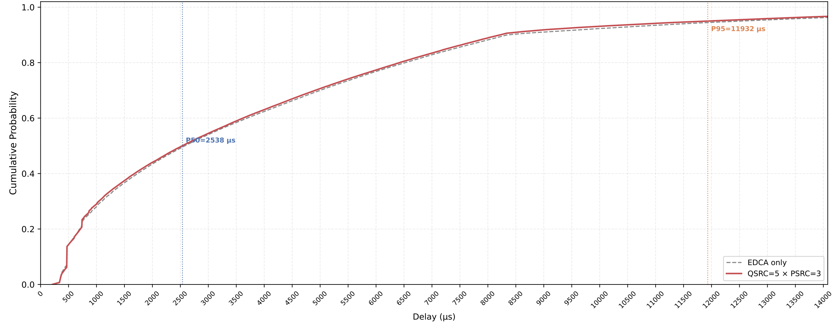
P-EDCA STA VO Delay CDF — QSRC=5 × PSRC=3 nSta=30, nPedca=15, 1Mbps, avg of 10 runs
